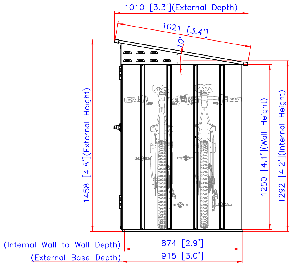
Side View
